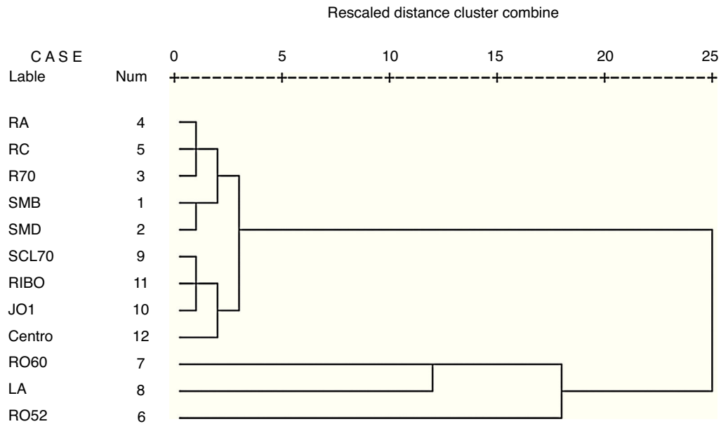
Fig. 1. Cluster analysis to identify cluster of antibodies in our sample of patients.
